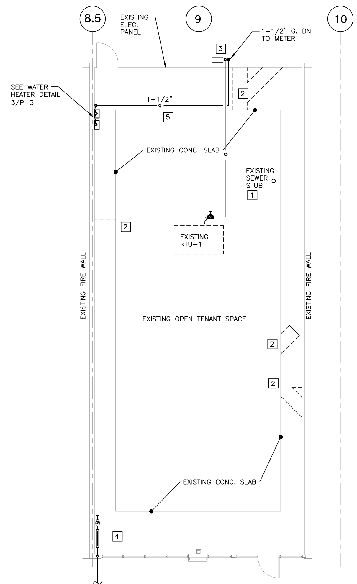
1 EXISTING FLOOR PLAN - PLUMBING 1/8" = 1'-0" NEW GAS PIPING SHOWN HERE ALSO
